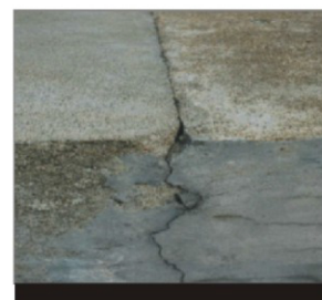
Construction joint Mạch ngừng
